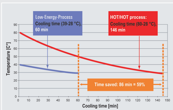
Comparison Low-Energy-Process vs. HOT/HOT Moisturizing cream, medium viscosity (O/W, 5000 liter, 42% fat phase)
