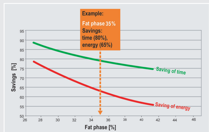
Saving potentials of Low-Energy-Process with various fat phases %
