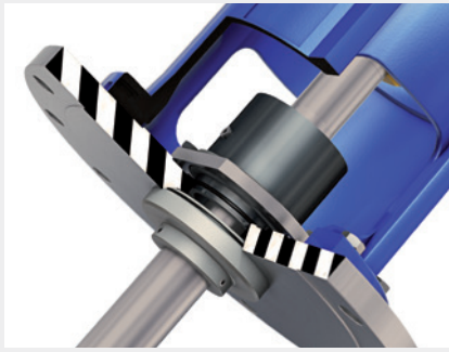
Shut-off device for mechanical seal maintenance during full tank
