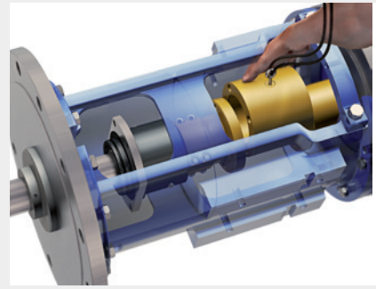
Advanced coupling design
