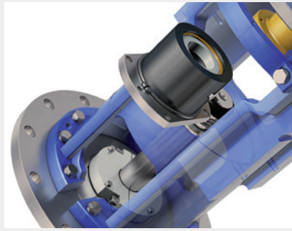
Single acting product lubricated mechanical seal easy to remove
