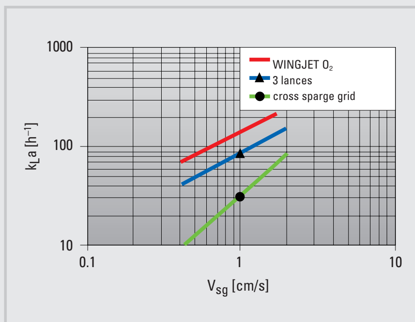
Oxygen mass transfer rate: k_{La} -value vs. superficial gas velocity. (Same operating data, agitator power and gassing rates)
