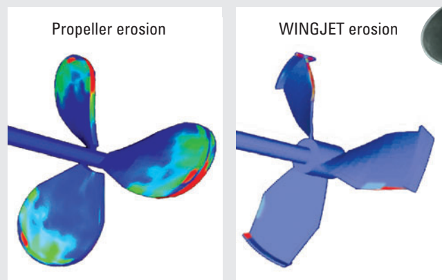
Comparison of areas exposed to wear on blade tips
